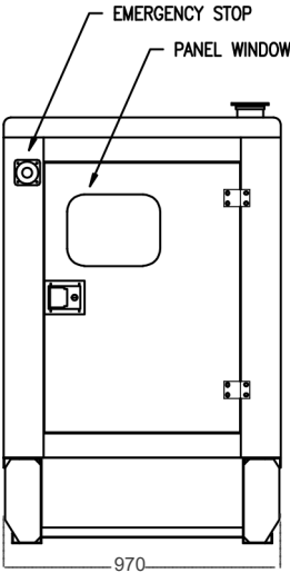
FRONT VIEW (ALTERNATOR SIDE)
